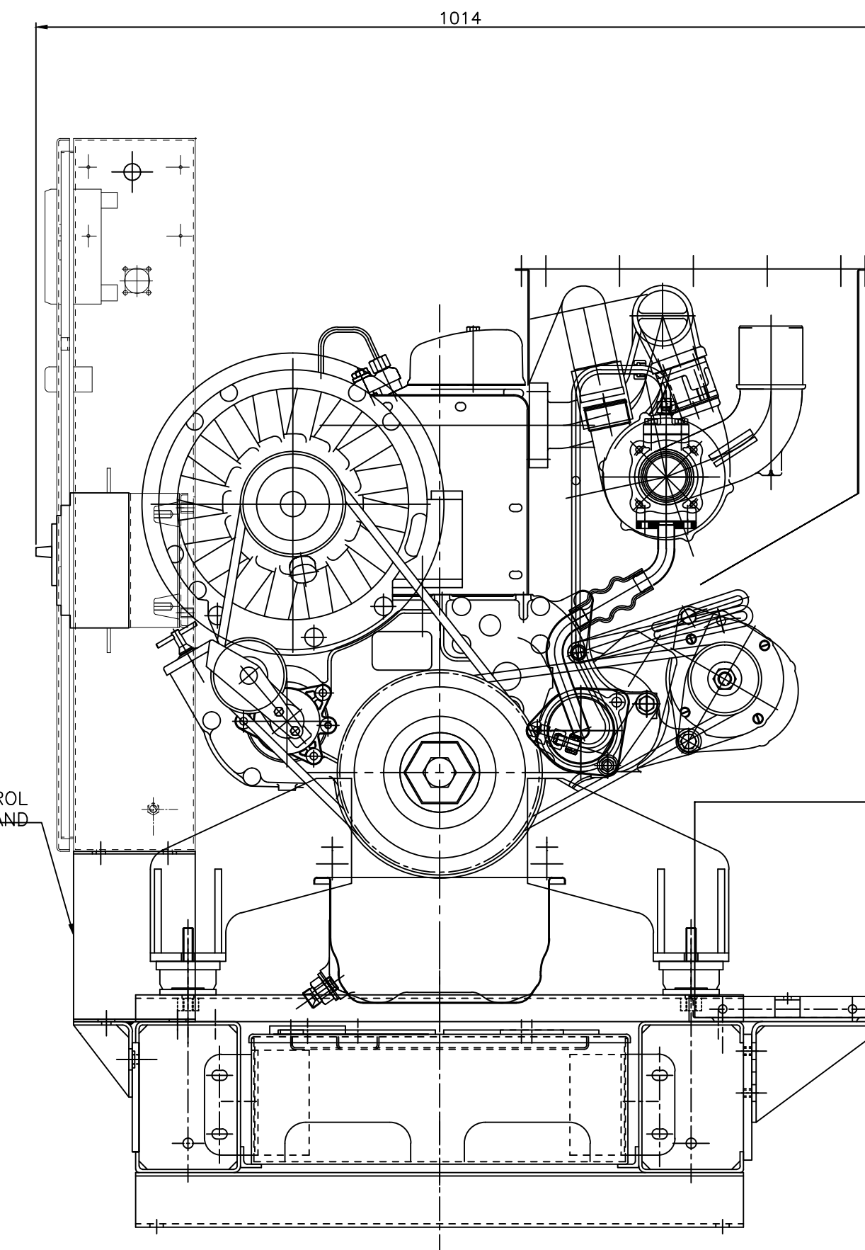
VIEW FROM GEAR END SIDE
